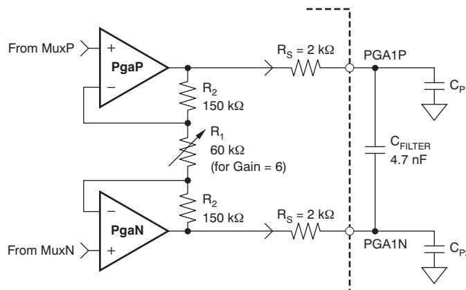
Figure 23. PGA Implementation
